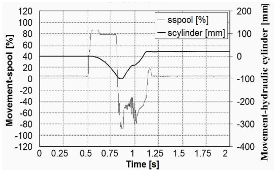
Fig. 9. Movement of the spool and the piston rod of the cylinder with the mass during the loading cycle in the water part of PCH
