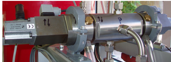
Fig. 4. The specimen – prototype of the proportional 4/3 directional control valve for water hydraulic
