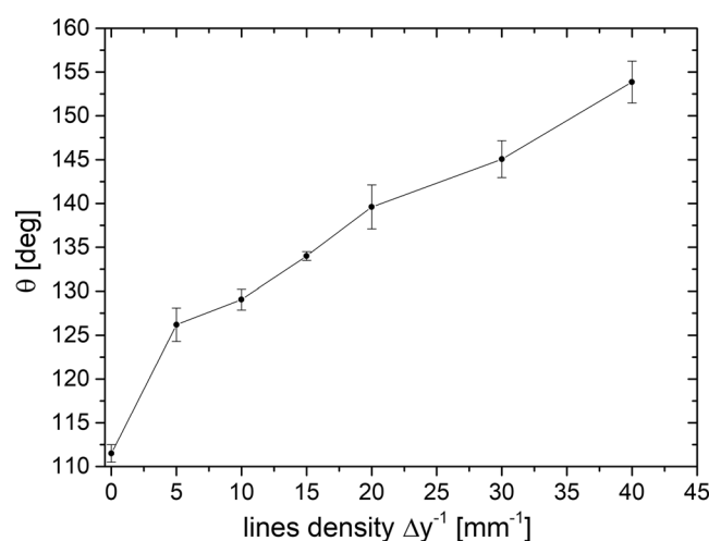
Figure 3. Change in the static water contact angle \theta as a function of increasing line density \Delta y^{-1} on a laser-textured AISI 316 L surface functionalized with 30-nm FAS-SiO 2 nanoparticles.
