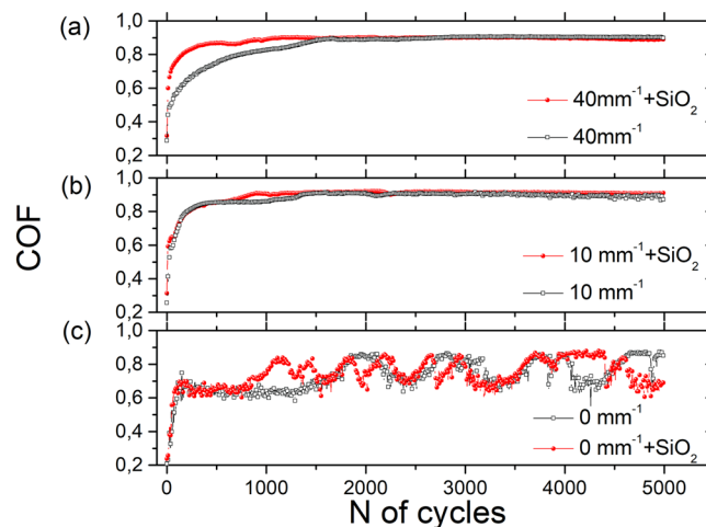
Figure 5. Typical COF lines for laser-textured AISI 316L surfaces without and with 30-nm FAS-SiO _2 nanoparticles in a dry environment. A clear difference in the running-in behaviour after adding nanoparticles is visible for samples with high \Delta y^{-1} (a), and no difference is observed for samples with low \Delta y^{-1} (b). For unprocessed samples (c), oscillations in the COF appear.
