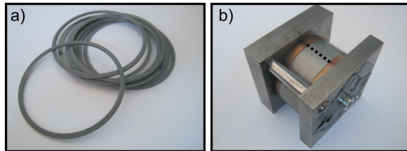
Fig. 3. a) typical shape of electrical laminations, and b) a clamping tool; here, the black dotted line shows the position of the weld
