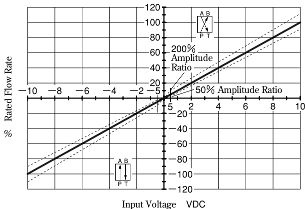
Fig. 9.8 Input Signal vs. Flow Rate
