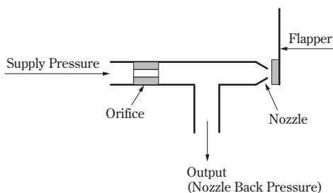
Fig. 9.16 Nozzle Flapper Mechanism
