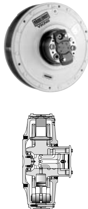
Fig. 10.9 Multi Stroke Radial Piston Motor
