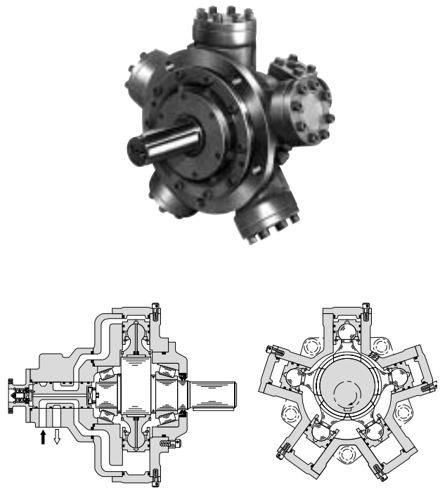
Fig. 10.8 Radial Piston Motor
